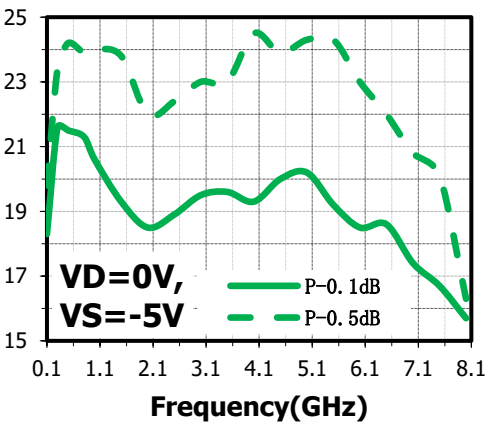
Bypass mode Input P -0.1/0.5 dB(dBm)
