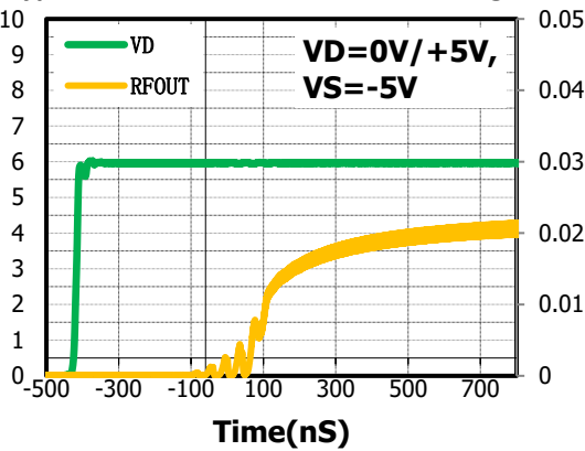
Bypass mode to Gain mode switching time
